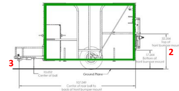
This sheet shows the UTV Calf-Catcher adjusted to the smallest dimensions
