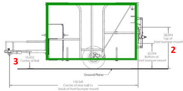
This sheet shows the UTV Calf-Catcher adjusted to the largest dimensions
