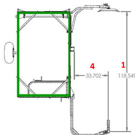
This sheet shows the UTV Calf-Catcher adjusted to the largest dimensions
